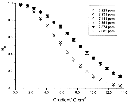
Figure 10: I/I 0 vs. Gi obtained from DOSY experiments on Co(II)(dmg) 2 .py.
